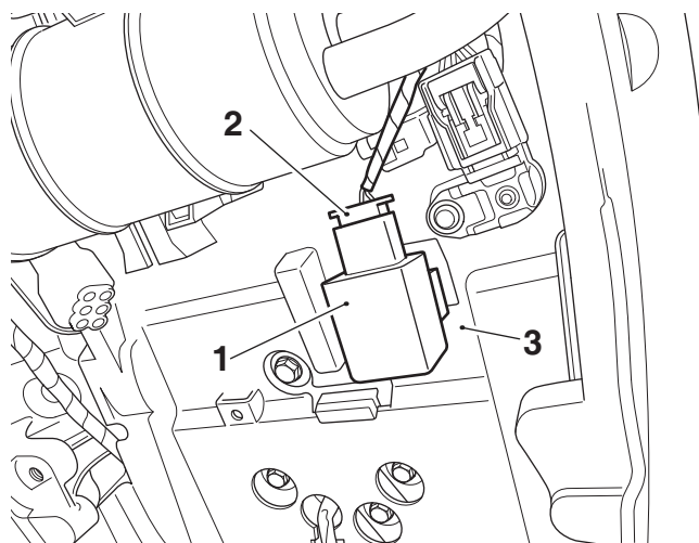
1. Indicator relay 2. Electrical connector 3. Undertray
