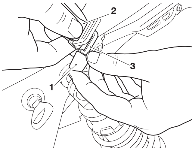
1. Webbing loop 2. Retaining strap 3. G-clip, inner section
